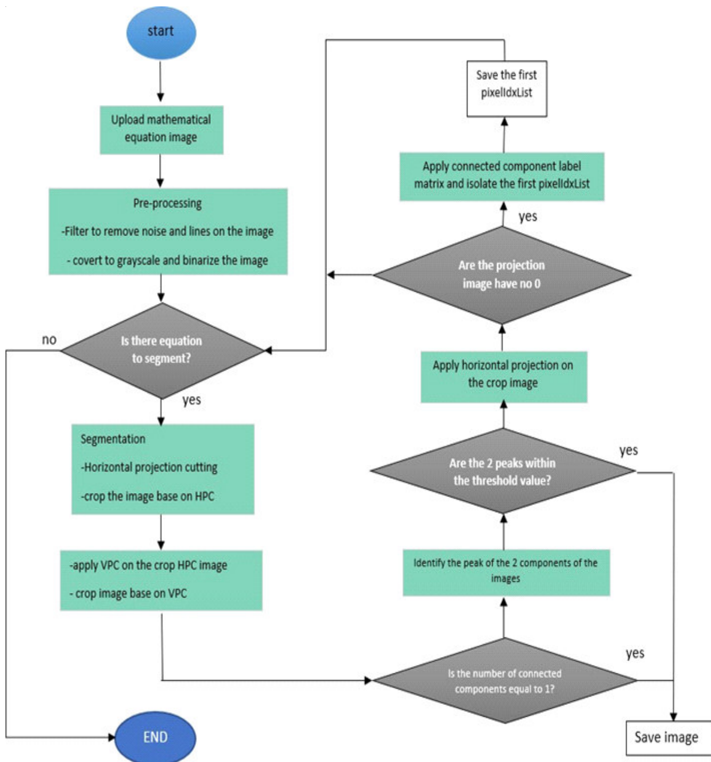
Figure 2. Flowchart of the Segmentation Algorithm
